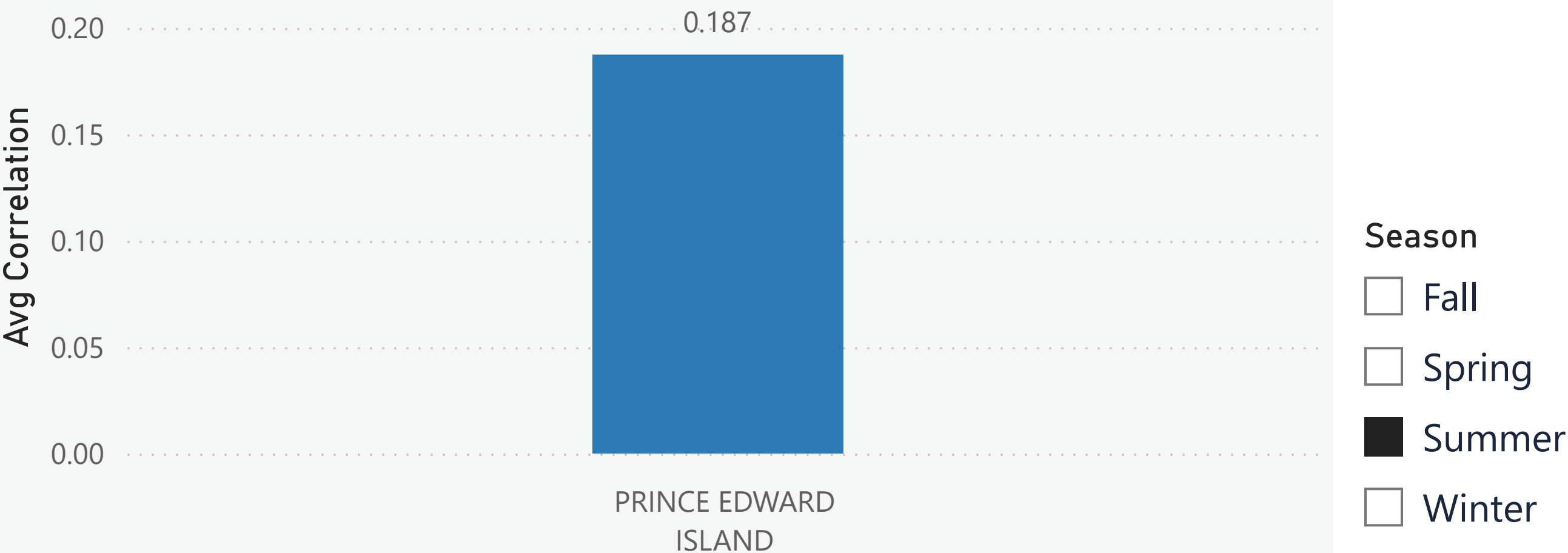
GHG Temperature Correlation
