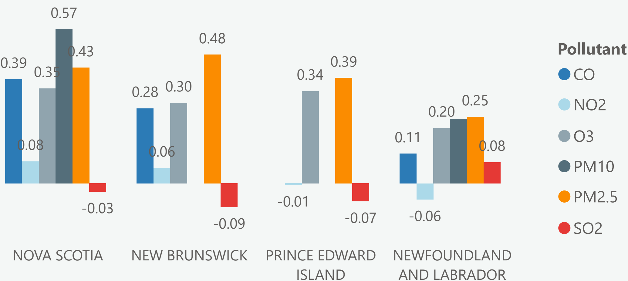
Pollutant Temperature Correlation
